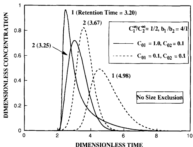
Figure 1. Peak reversal due to increased component 1 concentration.
