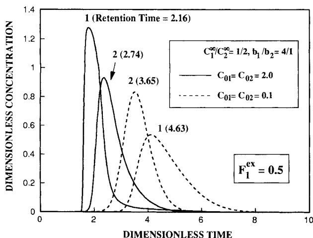
Figure 3. Peak reversal with size exclusion.
