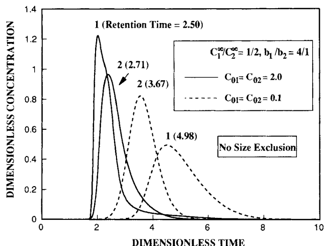
Figure 2. Peak reversal in binary elution without size exclusion.
