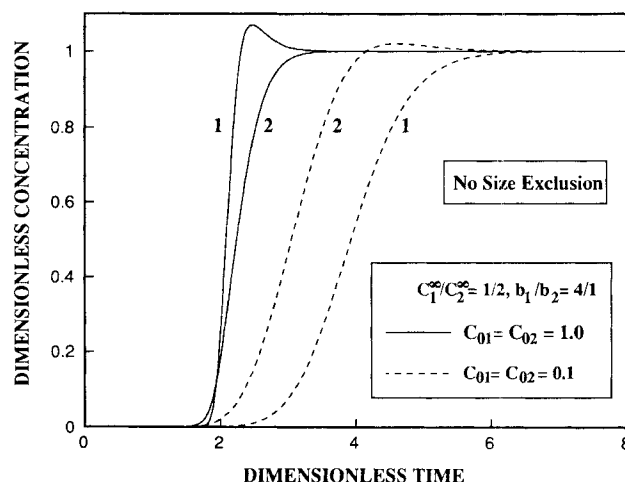
Figure 5. Crossover of breakthrough curves (no size exclusion).
